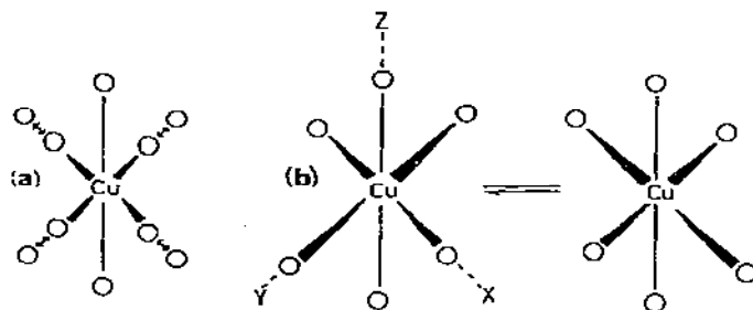
Fig. 18. Diagram illustrating two possible explanations of the unusual EPR parameters of K_3PbCu(NO_2)_6 ; (a) represents a vibronic mixing mechanism while (b) represents a rapid electron exchange between two tetragonally elongated molecules with orthogonal long axes.
