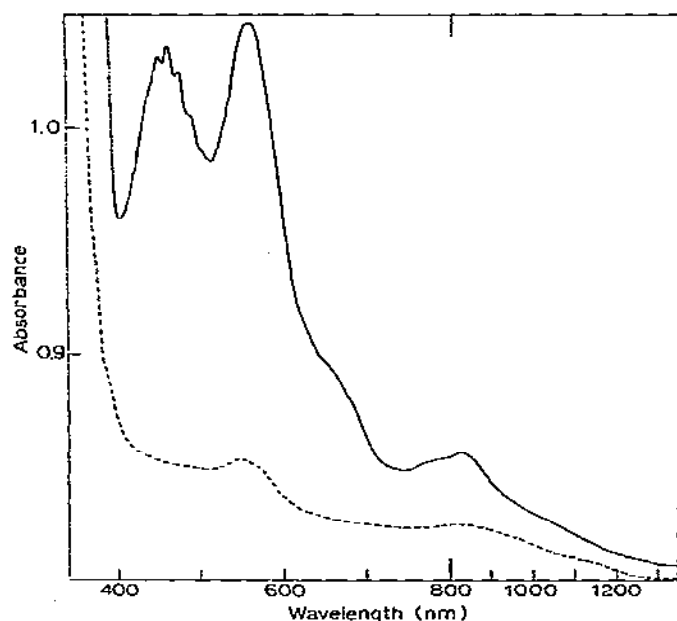
Fig. 17. Electronic spectrum of the (100) crystal face of [\text{Ni}(\text{4-mepy})_3(\text{NO}_2)_2]_2 \cdot 2 \text{C}_6\text{H}_6 with the electric vector along [010] (full line) and [001] (dashed line) measured at 7 K [43].
