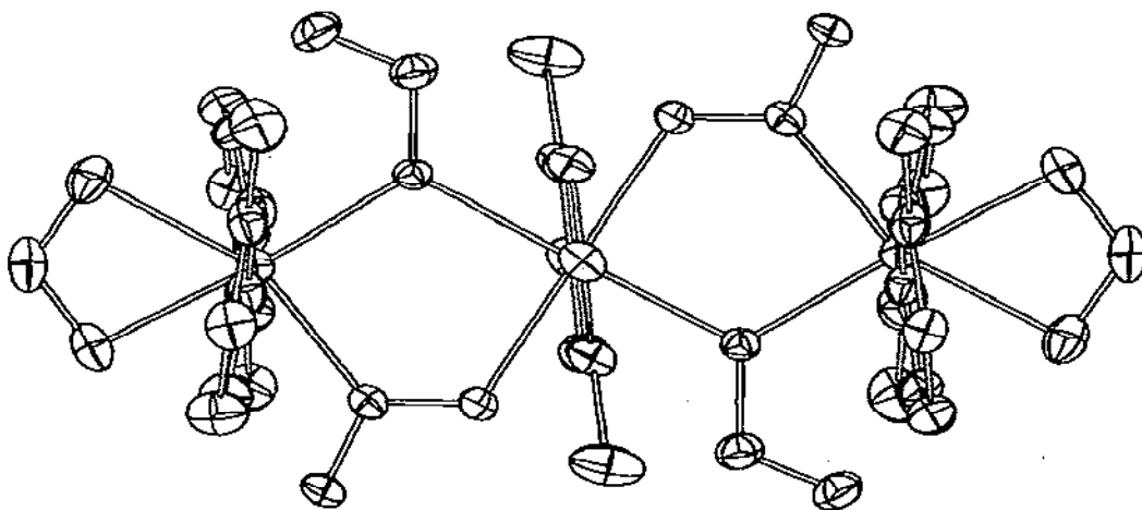
Fig. 7. Geometry of the trimer [\text{Ni}(\text{3-mepy})_3(\text{NO}_2)_2]_3 showing the plane containing the nitrite ligands [43].
