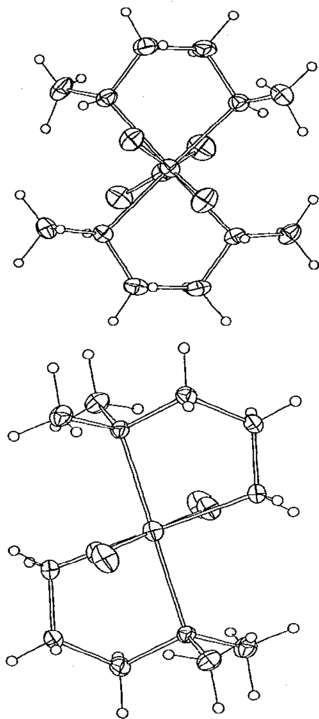
Fig. 3. Geometry of the molecules: (a) \text{Ni}(\text{NN}' \text{ dimen})_2(\text{NO}_2)_2 and (b) \text{Ni}(\text{NN dimen})_2(\text{ONO})_2 in each case looking down the metal-nitrite bond direction [14].
